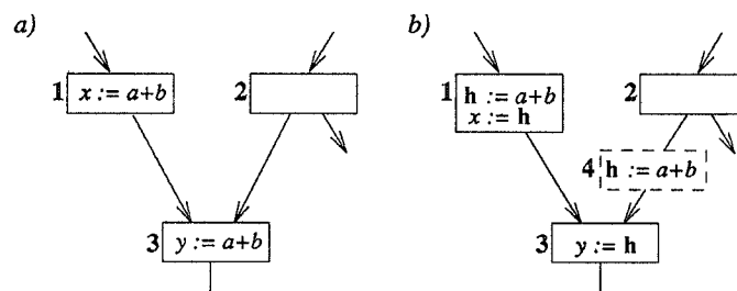
Figure 3: Critical Edges
